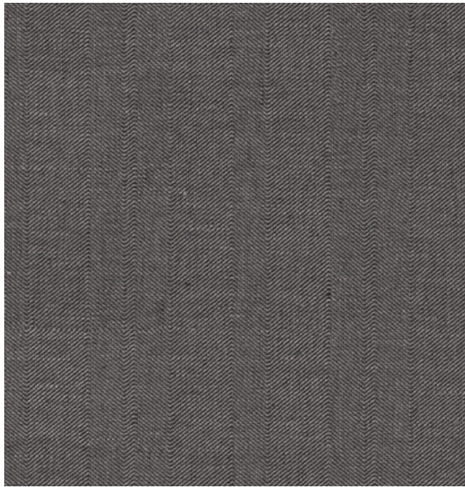
011 Singularity
