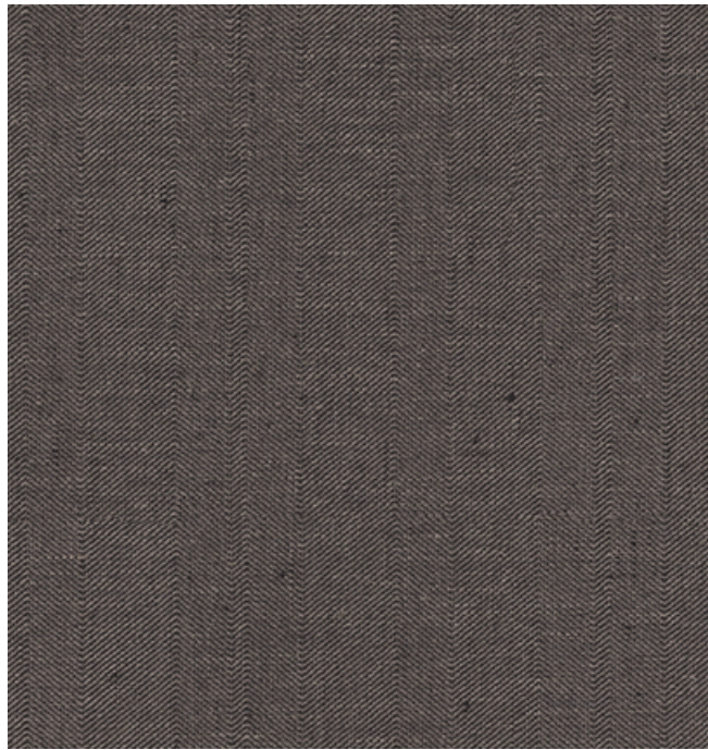
012 Universe
